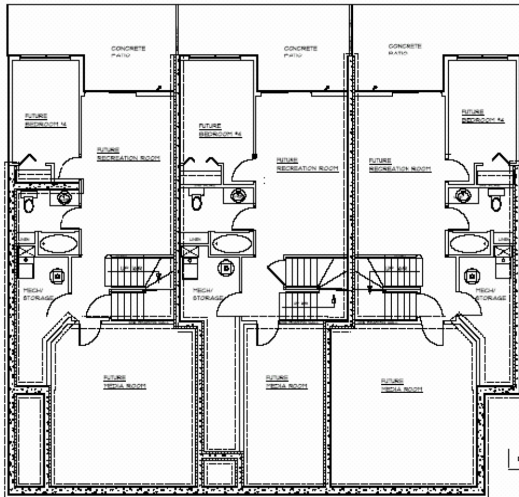
FOUNDATION PLAN UNIT #4
